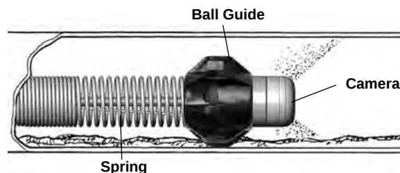
Figure 24 – Ball Guide In Use
