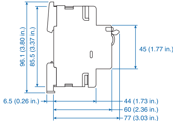
Dimensions in mm side view
