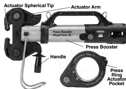
Figure 3 – MegaPress XL Ring and Press Booster/Z3 Actuator
