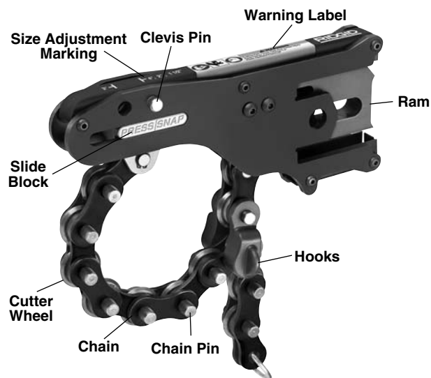
Figure 1 – Press Snap Soil Pipe Cutter
