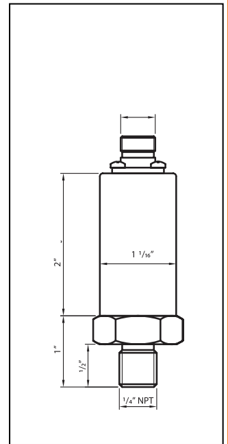
Fig 4: M12X1, 4-Pin
