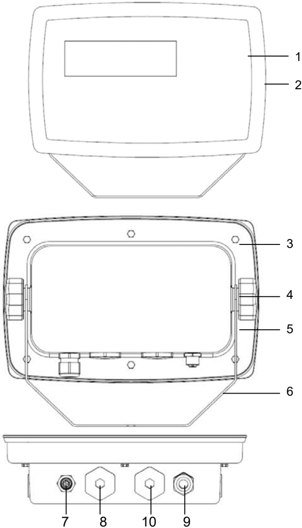
Figure 1-2 TD52XW Indicator
