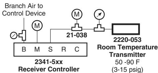
Figure 2 Typical Application.
