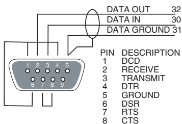
RS-232 DB-9 WIRING (VIEWED FROM WIRE SIDE)
