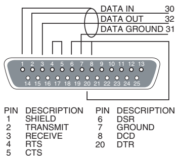
DB-25 WIRING (VIEWED FROM WIRE SIDE)
