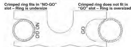
Figure 2 – Out of Tolerance Connections
