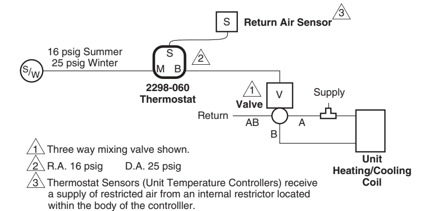
Figure 1 Typical 2298-060 and 2298-063 Summer/Winter Application.
