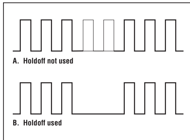
Fig. 4. Use of HOLDOFF Control.
