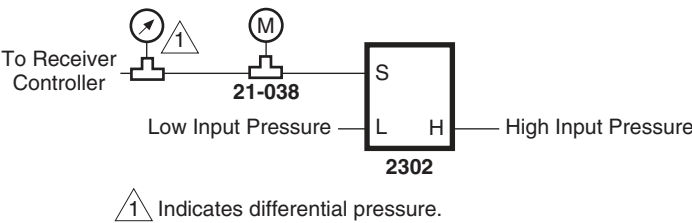
Figure 1 Piping Connections.
