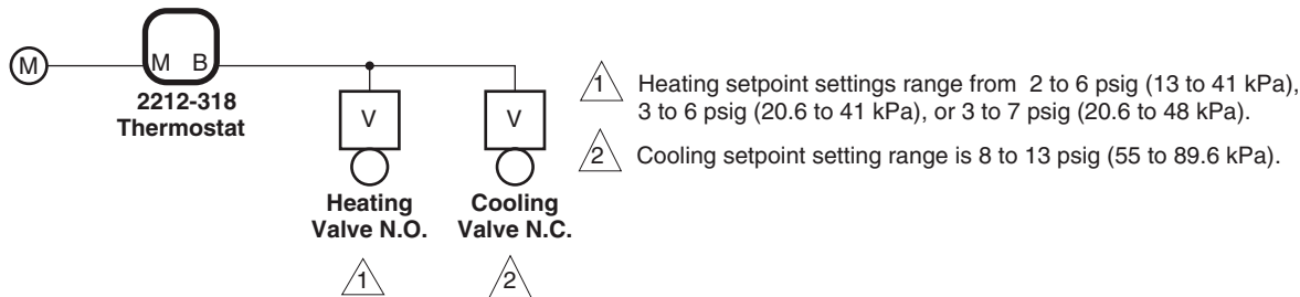
Figure 1 Typical Application.
