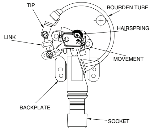
Figure 2A for link configuration of Type 1259 gauge.
