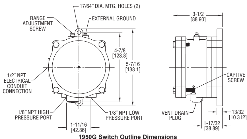
1950G Switch Outline Dimensions
