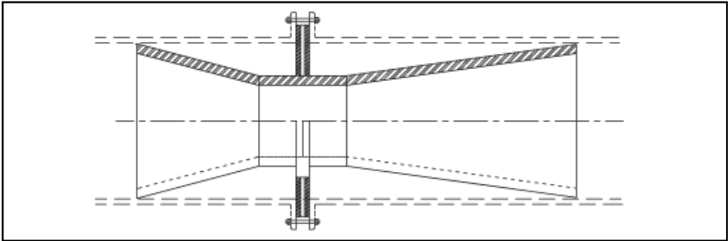
Fig 7: Insertion Type
