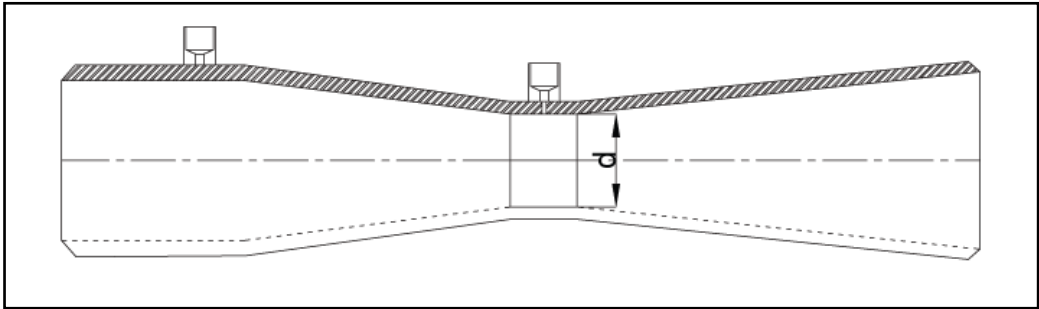
Fig 6: Weld-In Type
