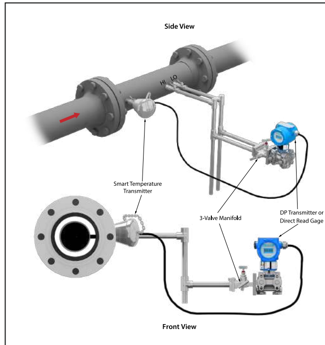
Fig 21: Vertical Installation for Steam
