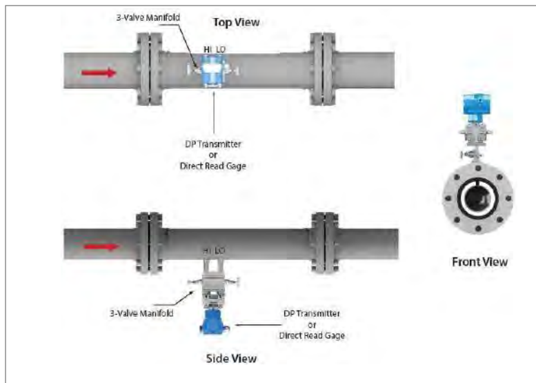
Fig 30: Horizontal Installation for Liquids
