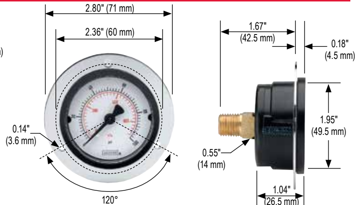
20-110 Front Flange
