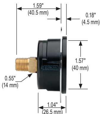
15-110 Front Flange
