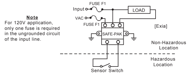
Fig. 1. Connection Diagram: Gems SAFE-PAK Models
