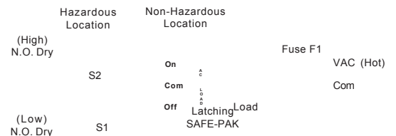
Fig. 2. Circuit for Pump-Down Operation
