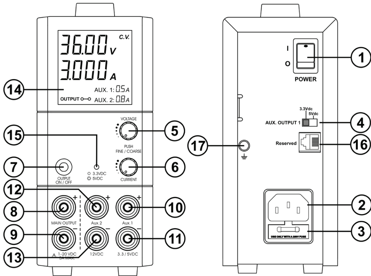
Figure 1 Panel Diagrams
