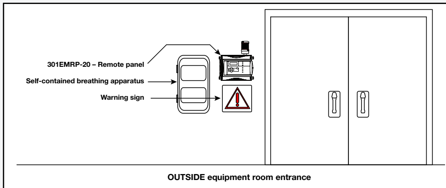
Figure 4 – Accessory layouts
