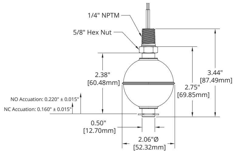
FS-400 Dimensions
