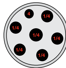
Multi-hole M05 (ATC-125 A/B)
