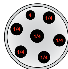
Multi-hole M05 (ATC-156/320/650 A/B / ITC-320/650 A)
