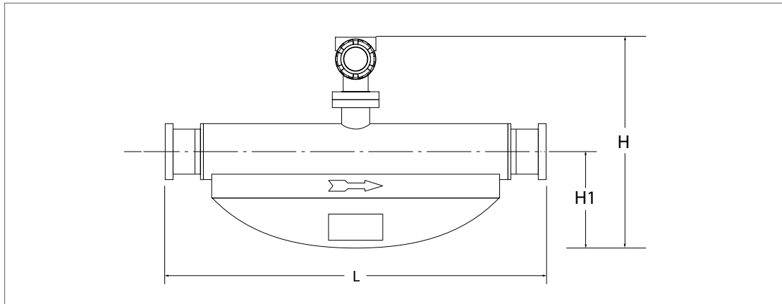
Super Bend sensor (Size \frac{3}{8} " to 8")
