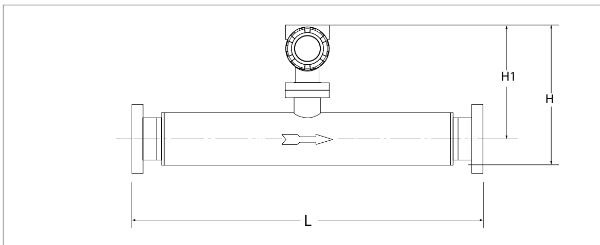
Straight sensor (Size \frac{3}{8} " to 1")
