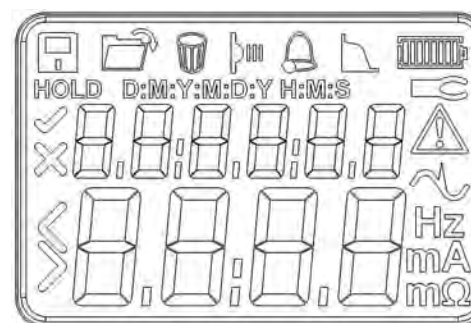
Figure 4: DET14C / DET24C Instrument Display View
