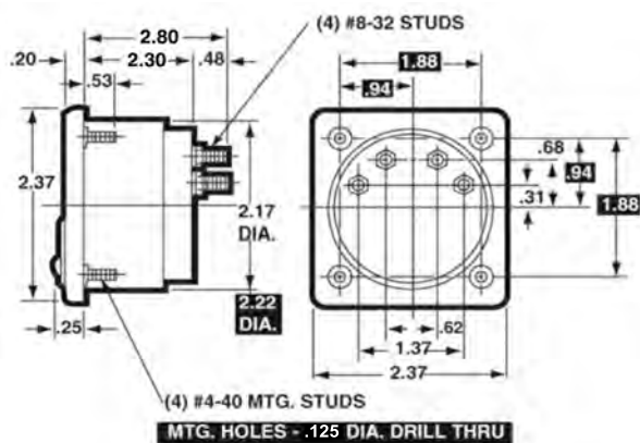
2-1/2" Model 177
