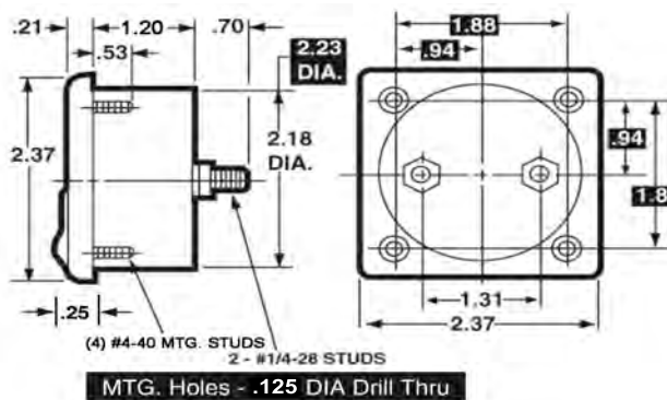
2-1/2" Model 127 & 127T, 147, 157, & 187
