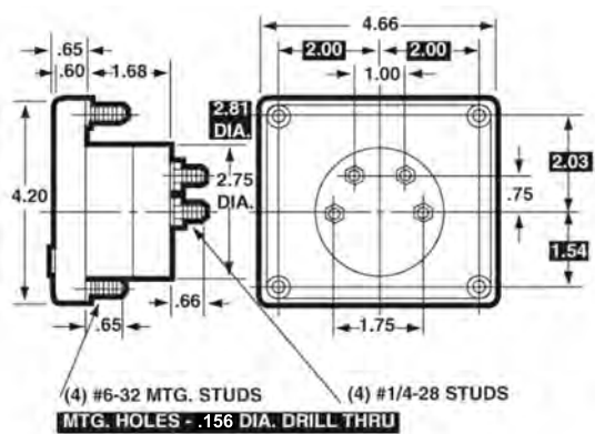
4-1/2" Model 79
