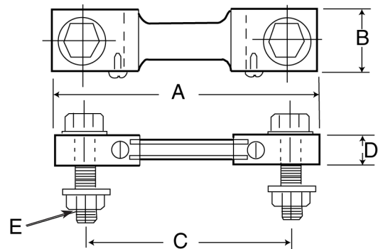
Switchboard Shunts
