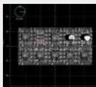
Pattern matching
